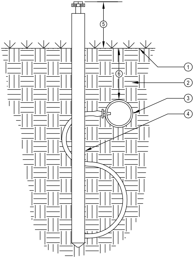
SECTION/ELEVATION NOT TO SCALE
