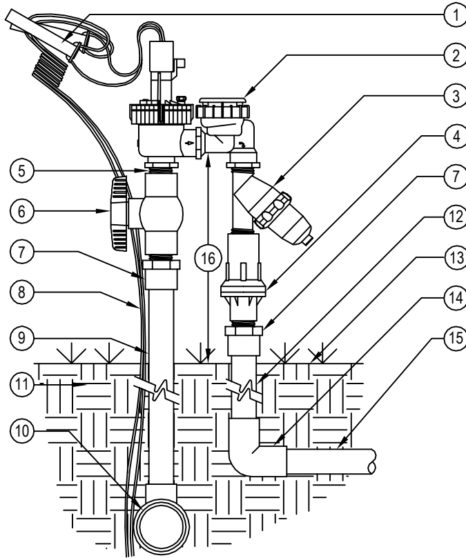
ELEVATION/SECTION NOT TO SCALE MIN. FLOW RATE - 2.0 GPM MAX. FLOW RATE - 20.0 GPM
