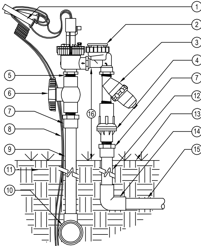
ELEVATION/SECTION NOT TO SCALE
