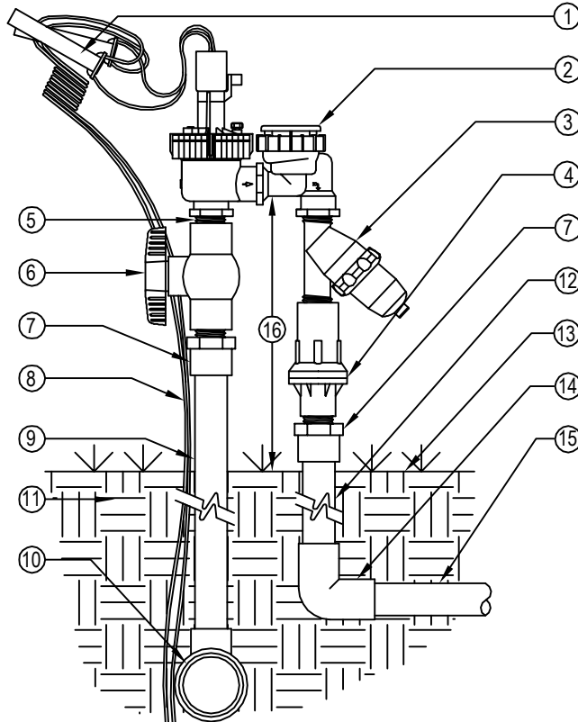
ELEVATION/SECTION NOT TO SCALE
