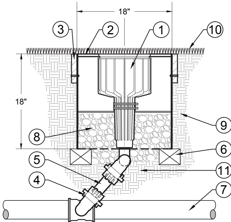
SECTION ELEVATION:
