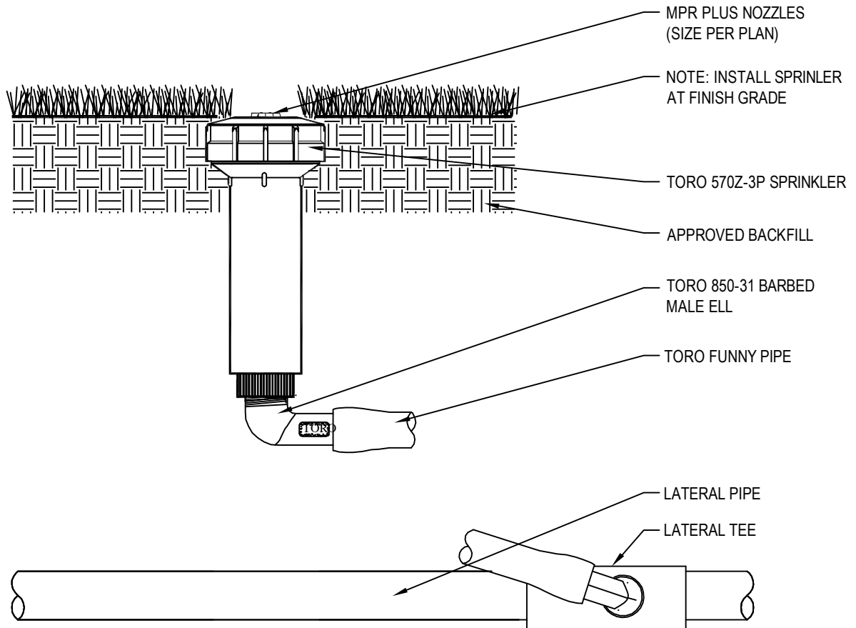
SECTION/ELEVATION
