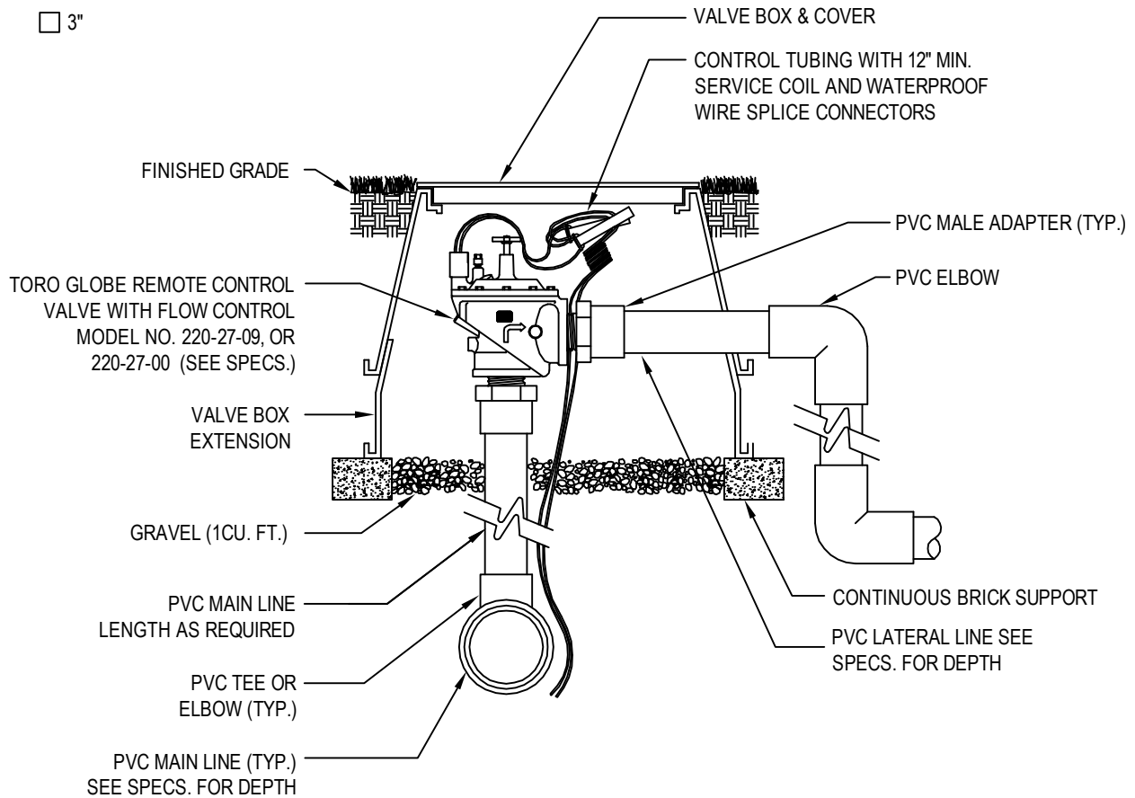
SECTION/ELEVATION
