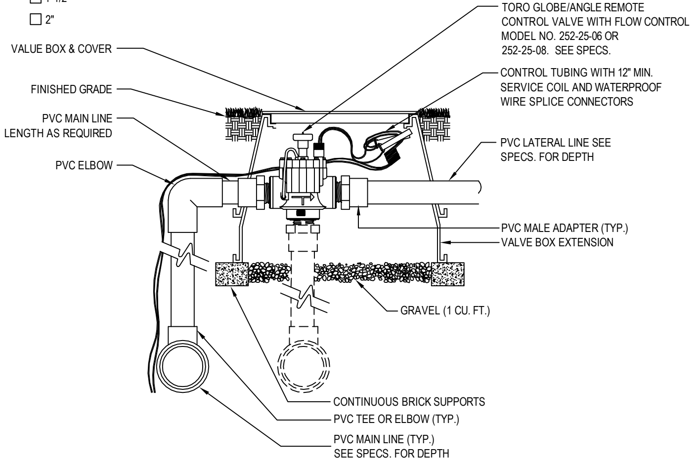
SECTION/ELEVATION NOT TO SCALE
